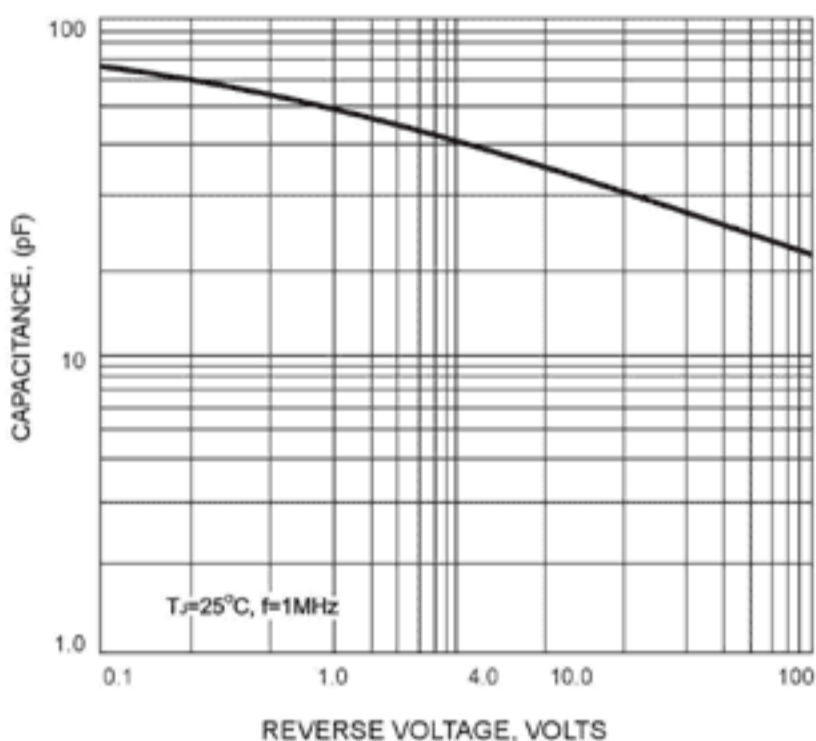
FIG. 3 - TYPICAL JUNCTION CAPACITANCE
