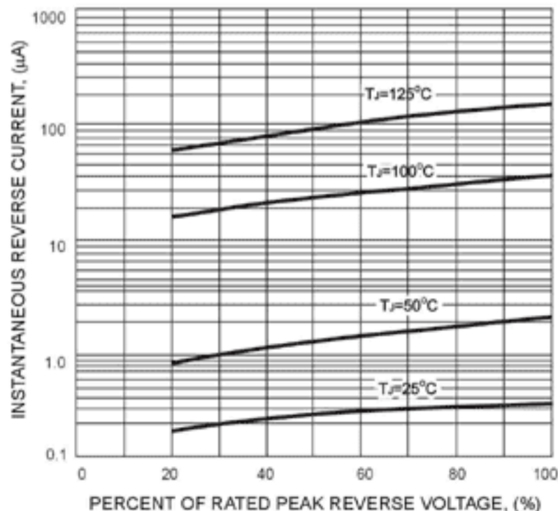
FIG. 5 - TYPICAL REVERSE CHARACTERISTICS
