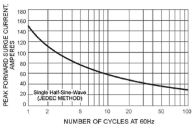
FIG. 1 - MAXIMUM NON-REPETITIVE SURGE CURRENT
