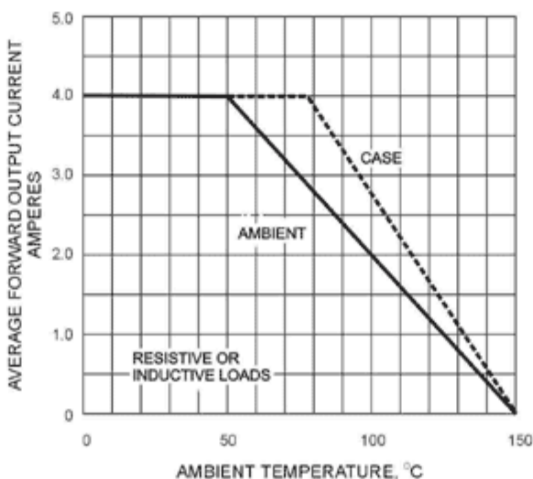
FIG. 2 - FORWARD DERATING CURRENT
