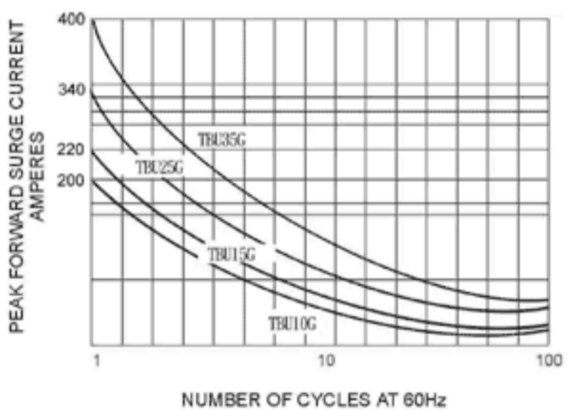
FIG. 1 - MAXIMUM FORWARD SURGE CURRENT
