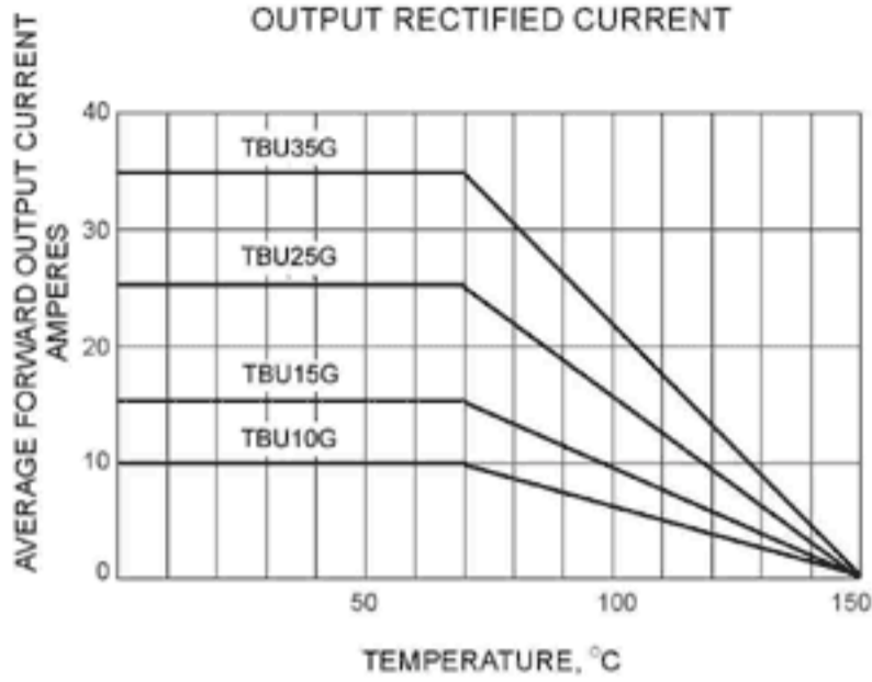
FIG. 2 - DERATING CURVE OUTPUT RECTIFIED CURRENT
